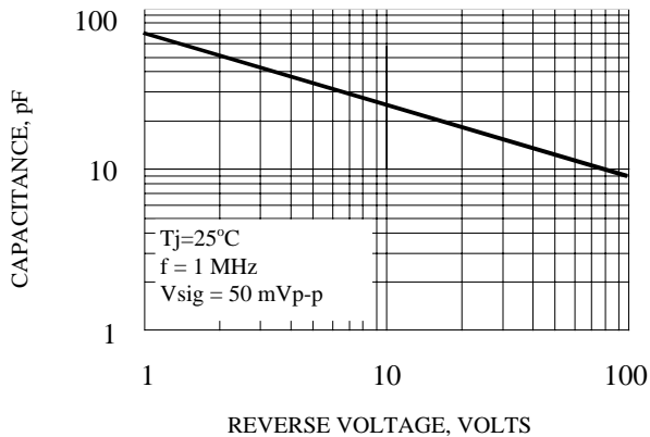
FIG. 5-TYPICAL JUNCTION CAPACITANCE
